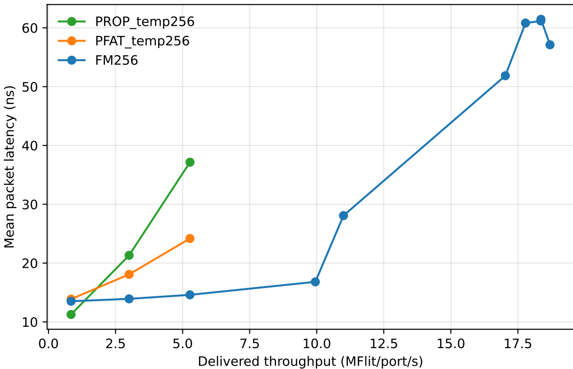
Fig.256-1 Three-DUT Global UR (tick=1)
